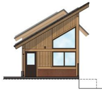
EAST ELEVATION
